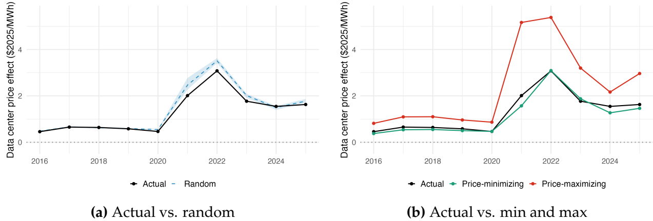
Figure 6: Cumulative data center wholesale price effects
