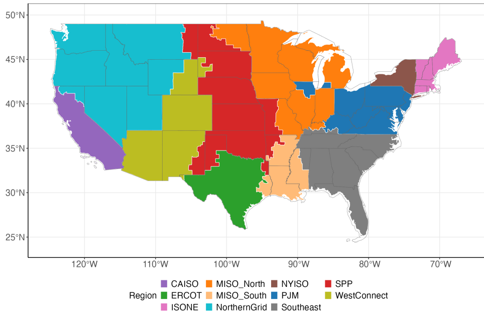
Figure B.10: Dispatch model regions
