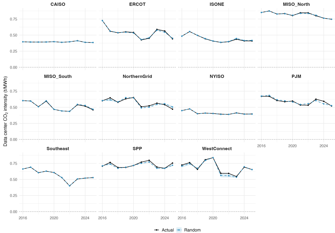
Figure B.17: Marginal emissions intensity of data center load, by region
