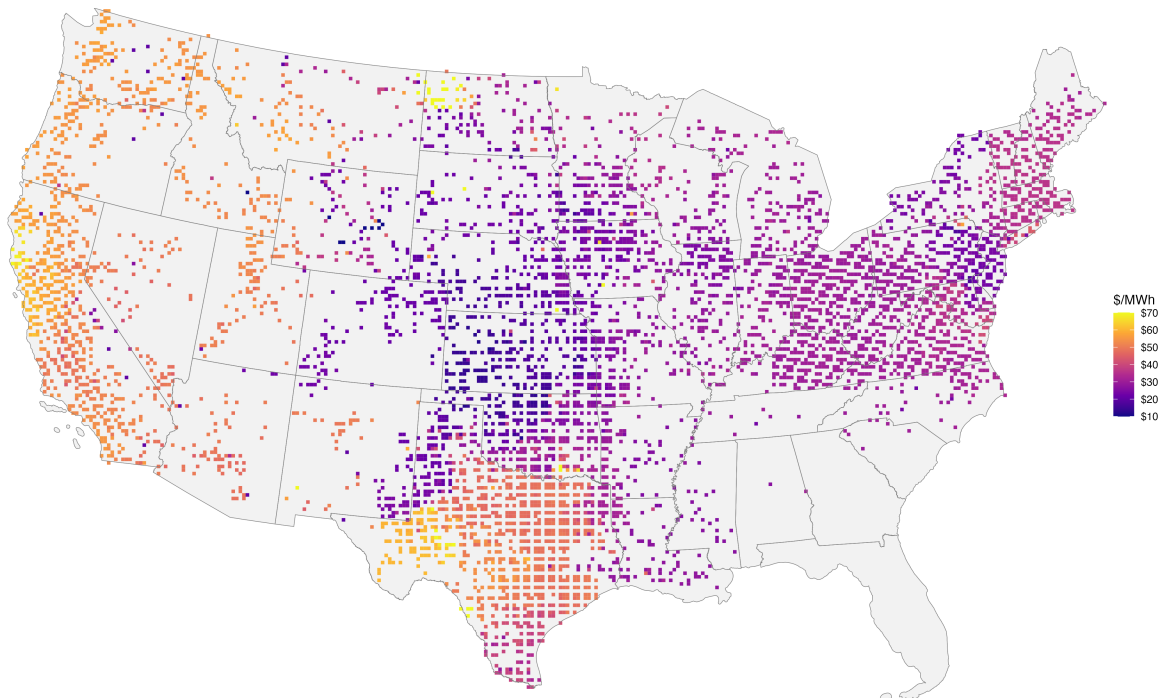
Figure B.6: LBNL gridcell wholesale prices, 2023
