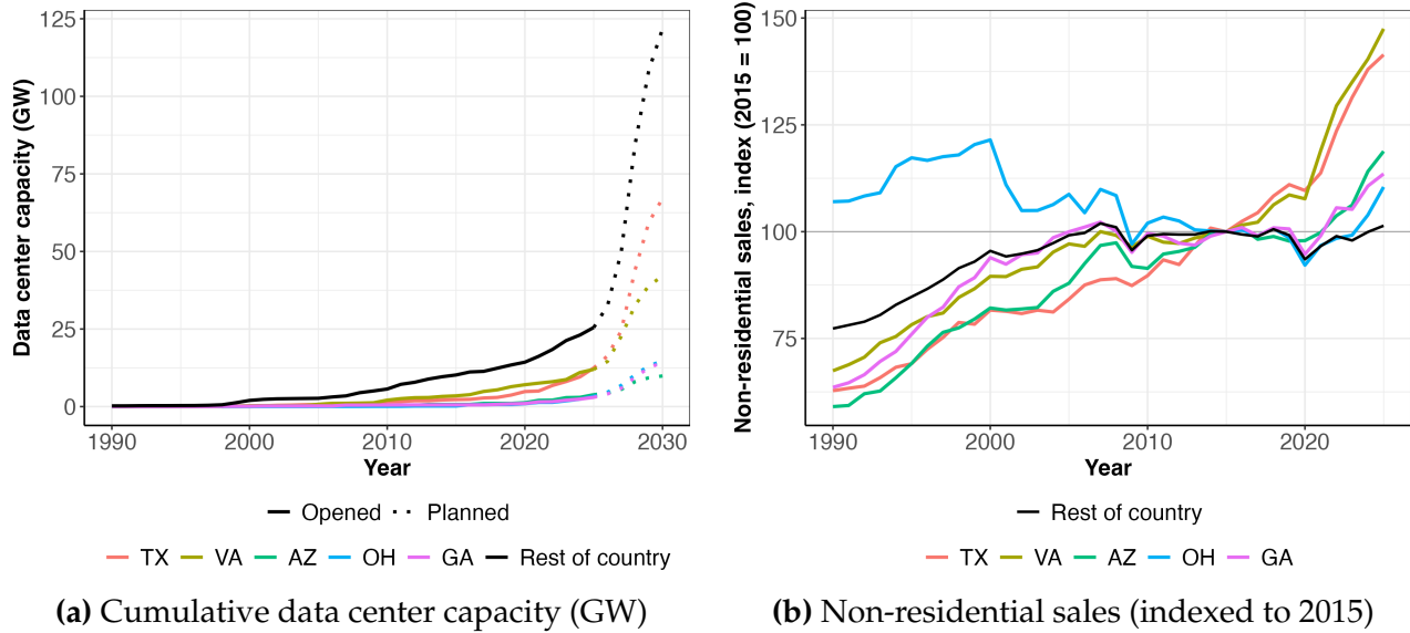
Figure 2: Data center capacity and non-residential sales for the top states by data center growth
