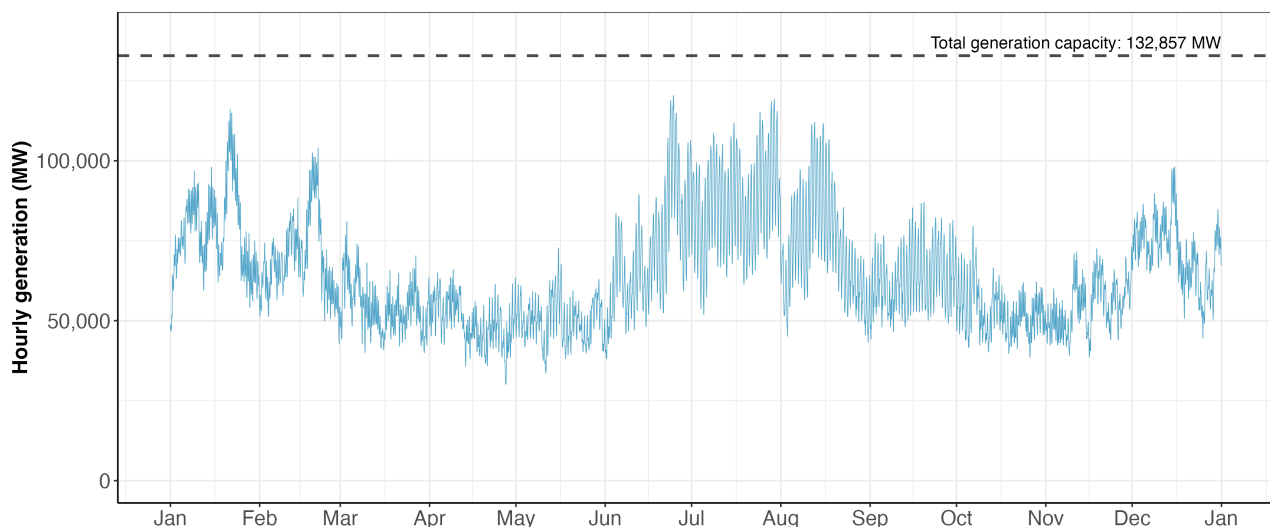
Figure B.9: PJM’s hourly generation and total capacity, 2025
