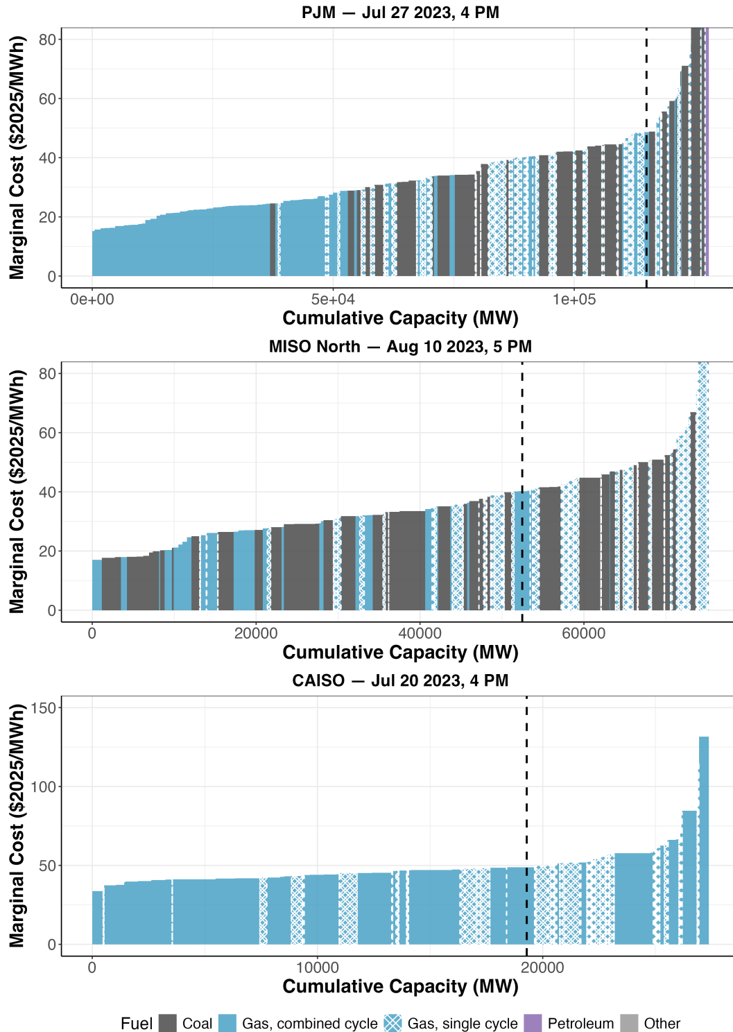
Figure B.12: Example supply curves
