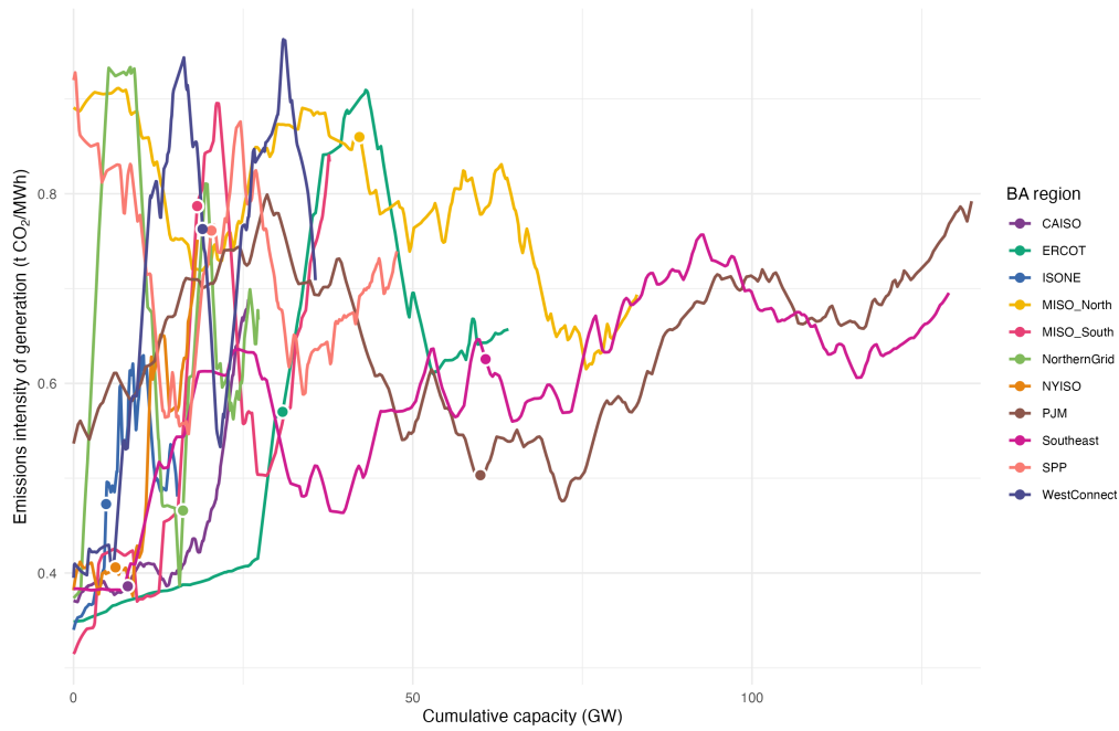
Figure B.3: 2019 regional dispatch supply curves: marginal emissions intensity
