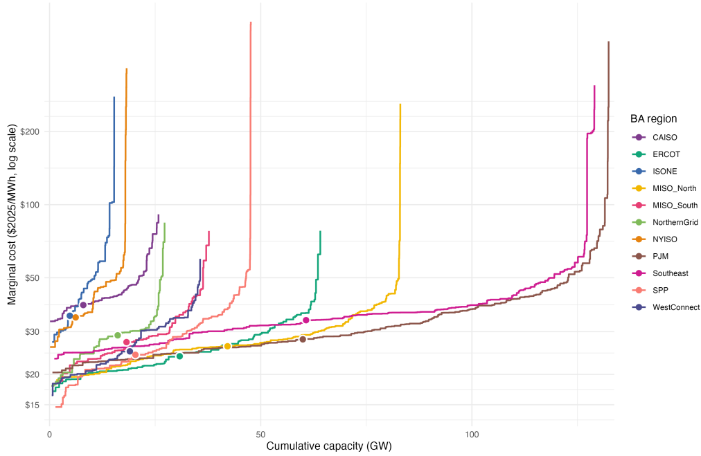
Figure 4: 2019 regional dispatch model supply curves
