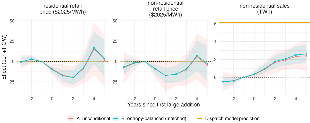
Figure 8: Local projections DiD: retail price and load effects of data center entry, across-region controls
