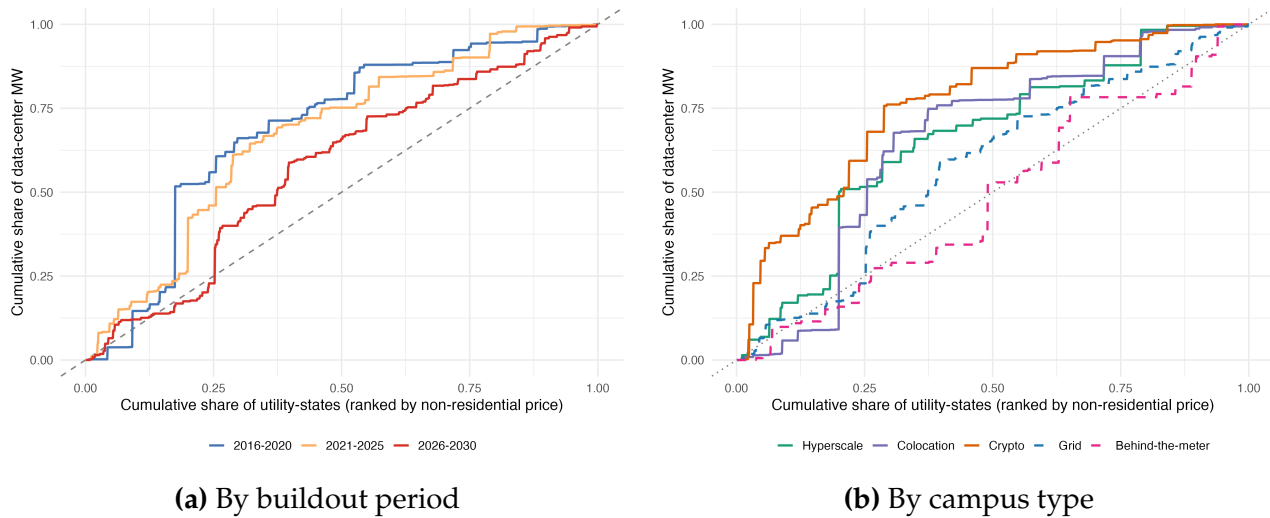
Figure B.21: Data center capacity concentration by non-residential price
