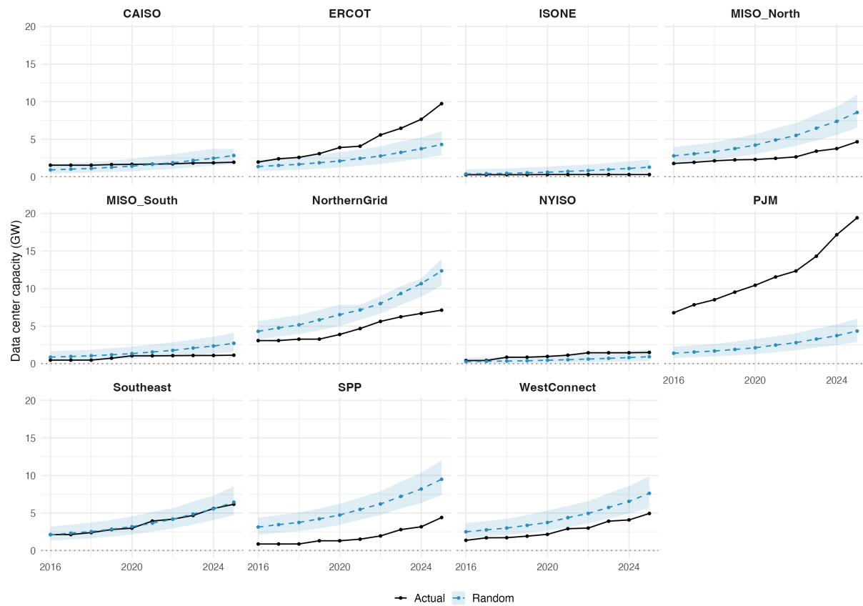
Figure B.14: Cumulative data center capacity by region
