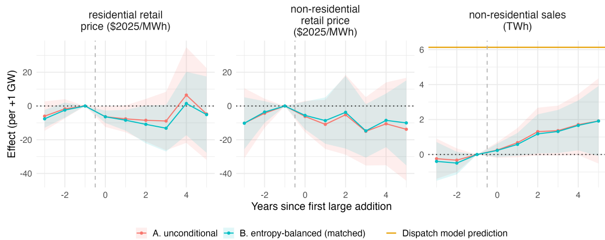
Figure B.19: Local projections DiD: retail price and load effects of data center entry, within-region controls
