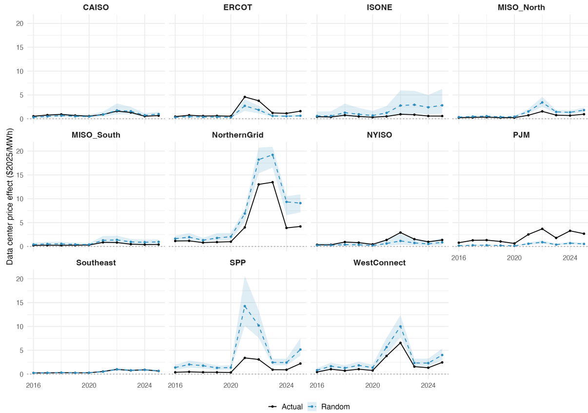
Figure B.15: Data center-induced wholesale price effect by region
