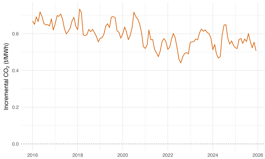
Figure B.16: National marginal emissions intensity of data center load
