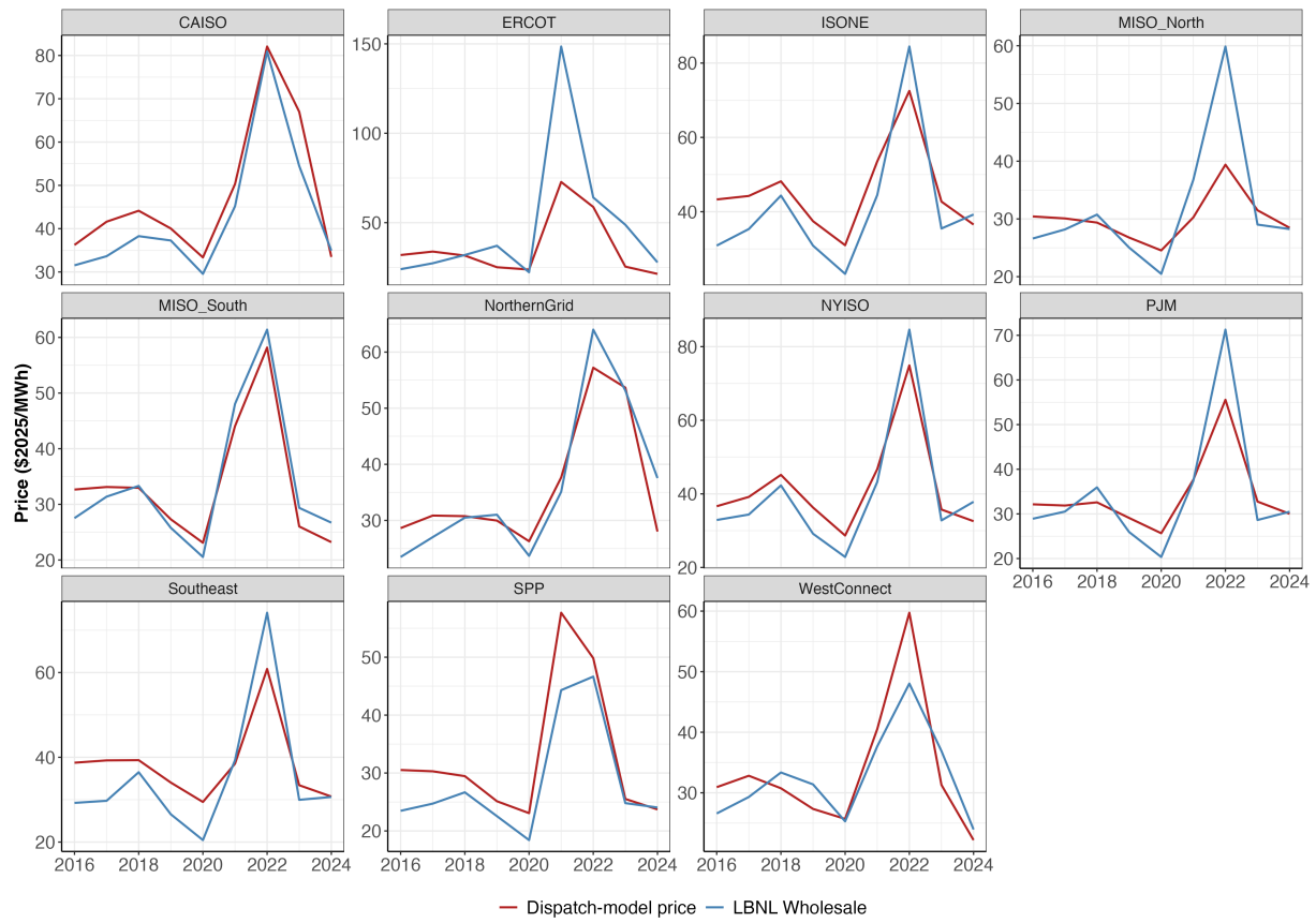
Figure B.13: LBNL wholesale prices vs. modeled prices by region
