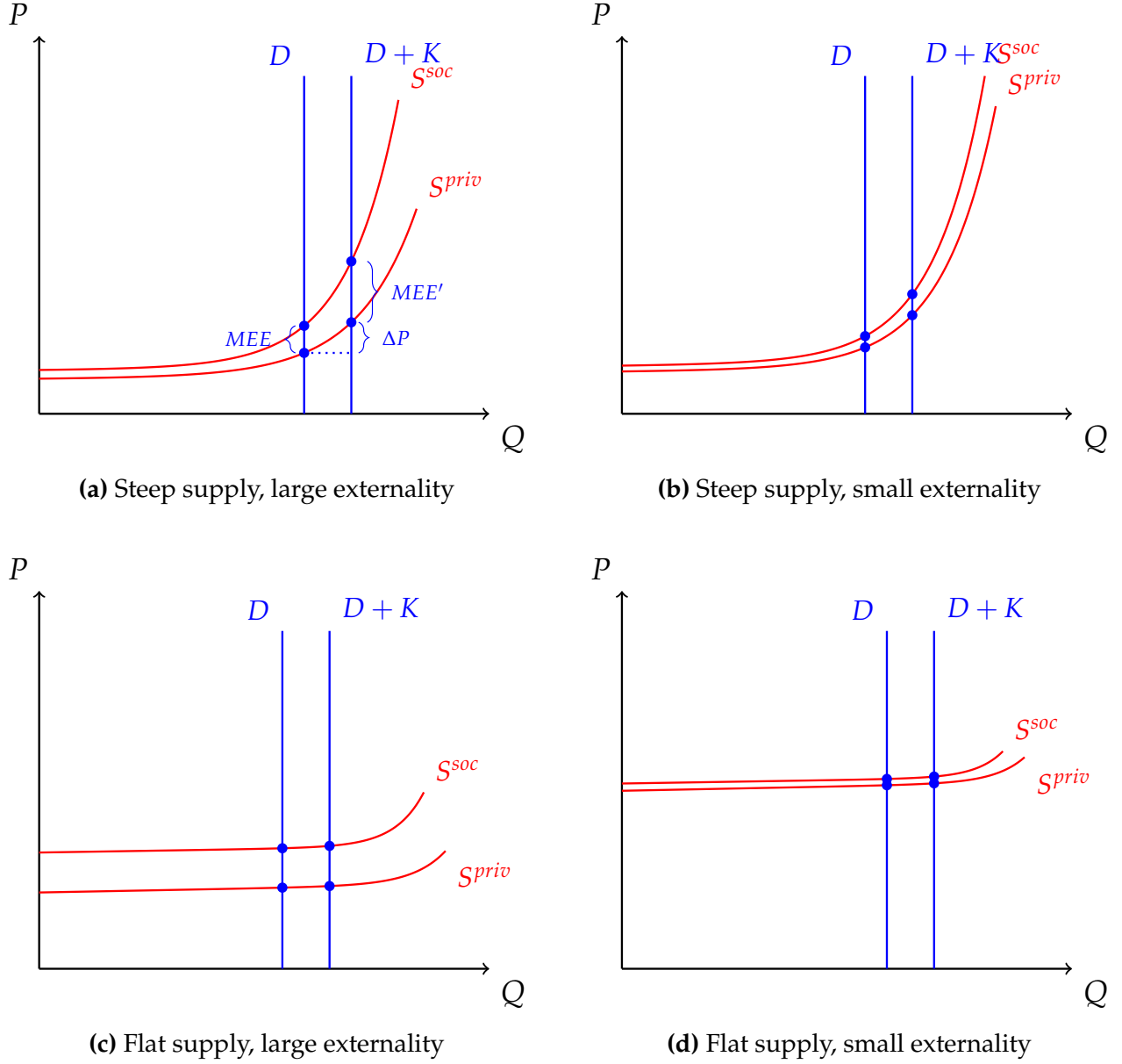
Figure 1: Stylized impacts of data center demand on emissions and prices
