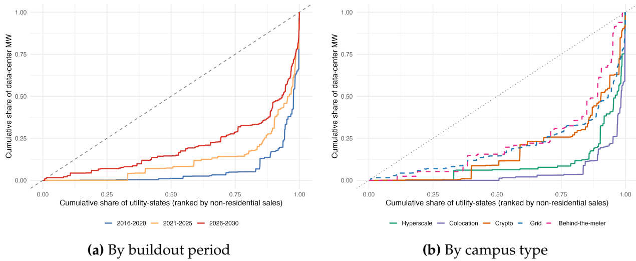
Figure B.22: Data center capacity concentration by non-residential sales
