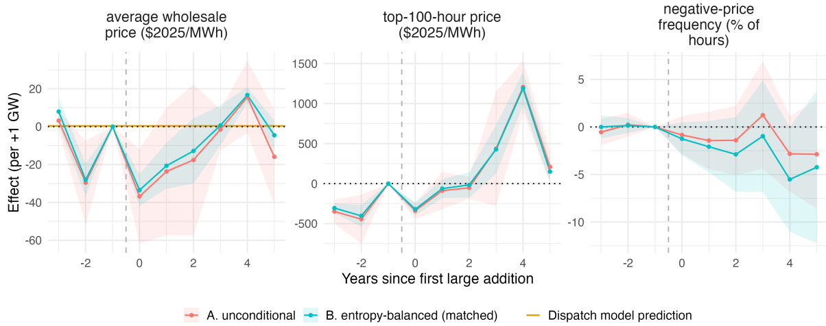
Figure B.20: Local projections DiD: wholesale price effects of data center entry
