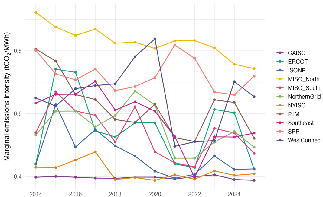
Figure B.5: Marginal emissions intensity by region and year
