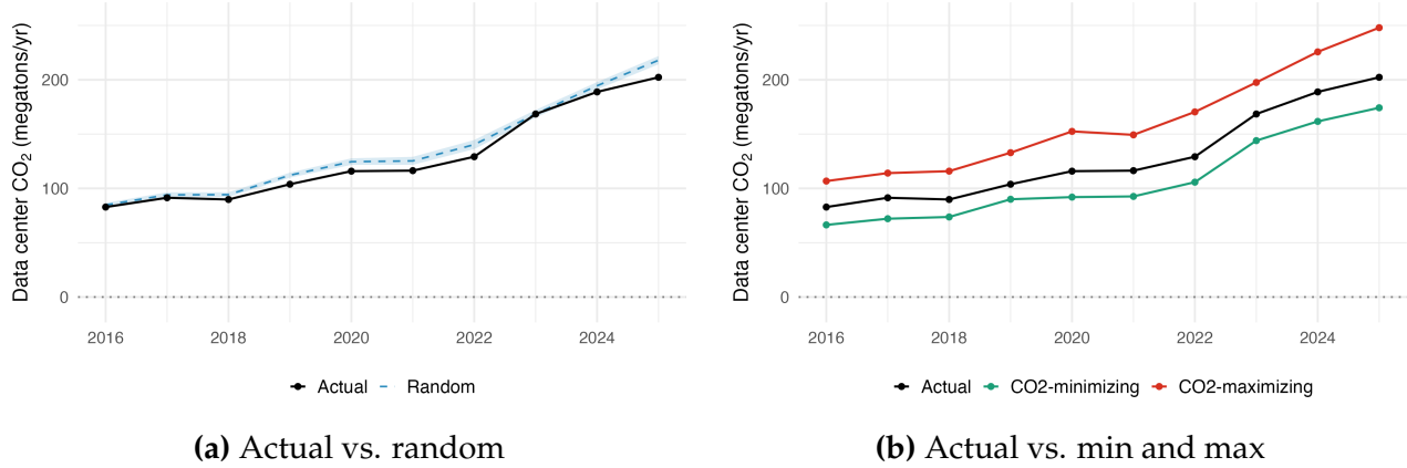
Figure 7: Cumulative data center emissions effects
