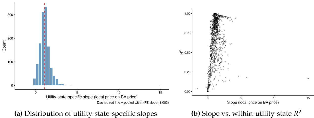
Figure A.1: Utility-state-specific fit of local MCPs on regional MCPs
