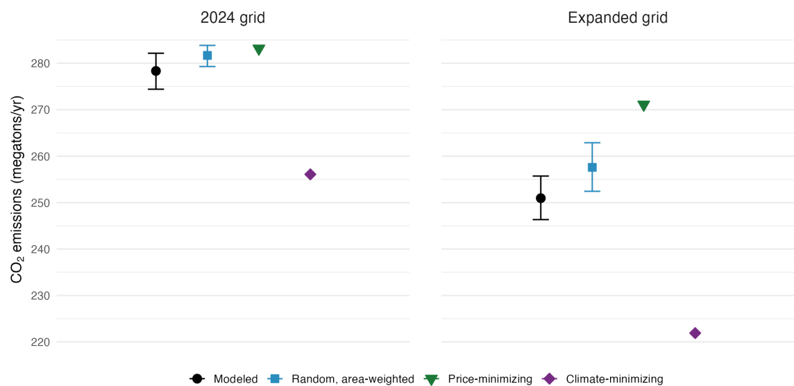
Figure B.25: Incremental emissions by data center allocation, 2024 grid and augmented grid (2026–2030 buildout, 50% realization)
