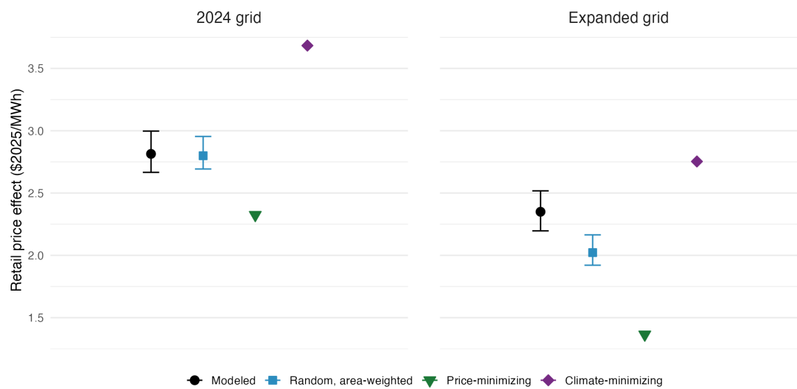
Figure B.24: Retail price effect by data center allocation, 2024 grid and augmented grid (2026–2030 buildout, 50% realization)
