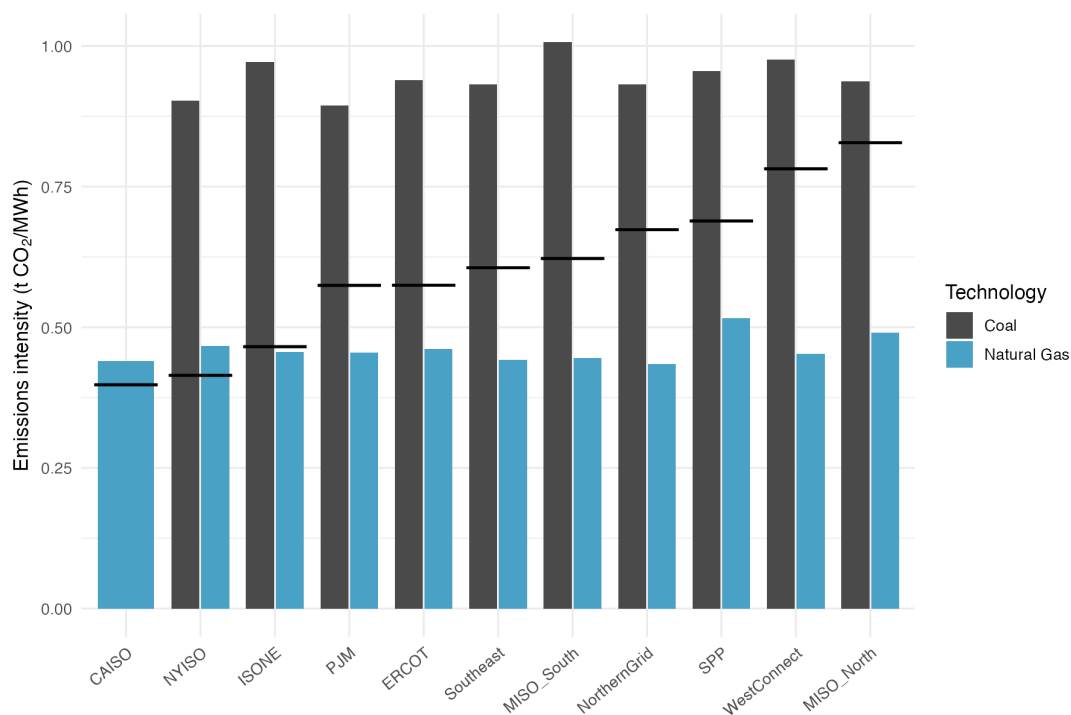
Figure B.11: Marginal emissions intensity vs. coal and gas fleet intensity, by region
