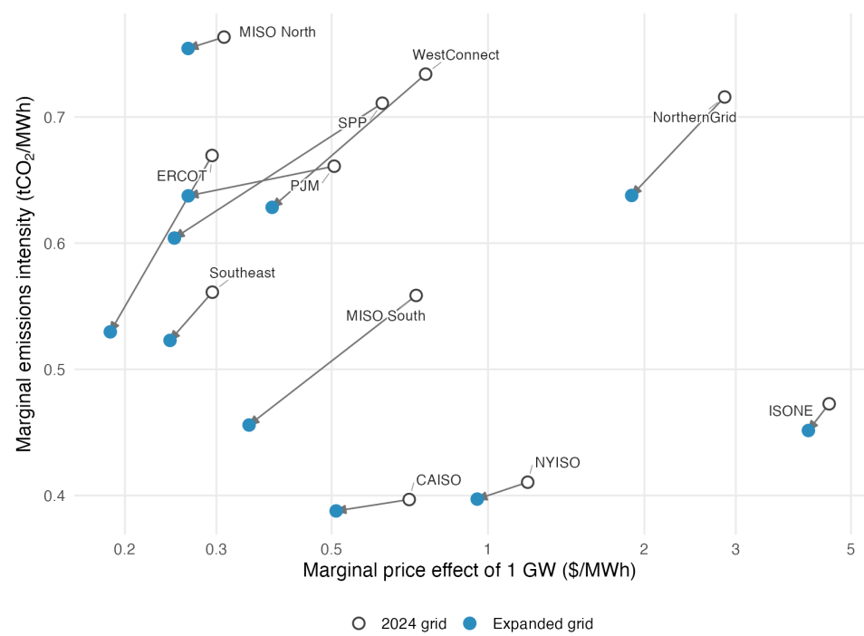
Figure B.26: Marginal price and emissions effects of added load by dispatch region, 2024 grid and augmented grid
