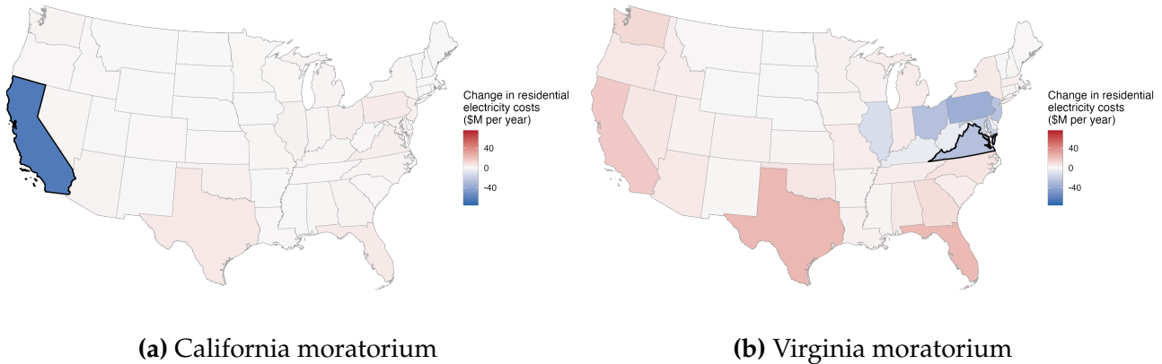
Figure 9: Change in residential electricity costs by state under a California or Virginia data center moratorium (2021–2025 buildout)
