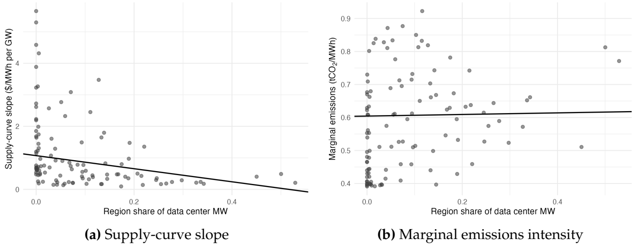
Figure 5: Data center concentration and grid characteristics
