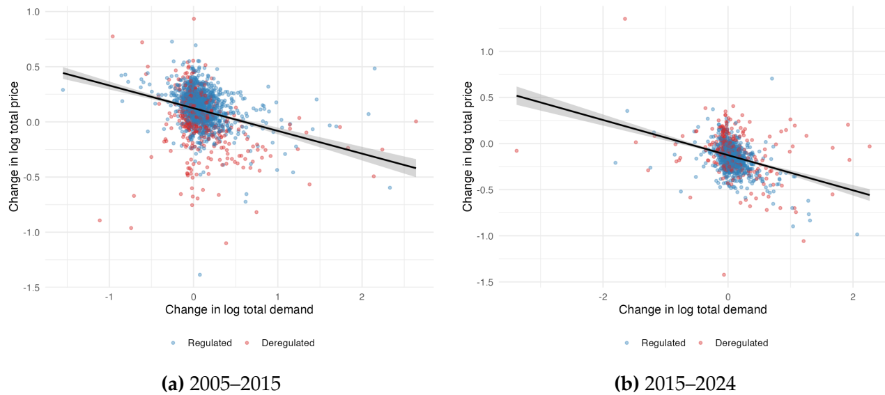
Figure B.8: Total demand and price changes across utility-states
